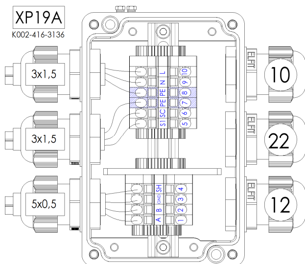
1x 230VAC, 1x relay (max 10A/250VAC), DATA (PDE)
