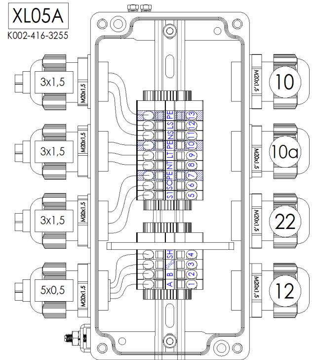
1x 230V, 1x 230VAC (heating), 1x relay (max 10A/250VAC), DATA (PDE)
